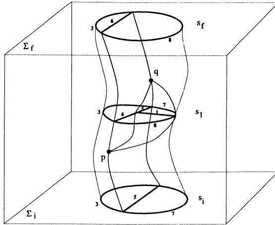
Figure 4: A term of second order.
