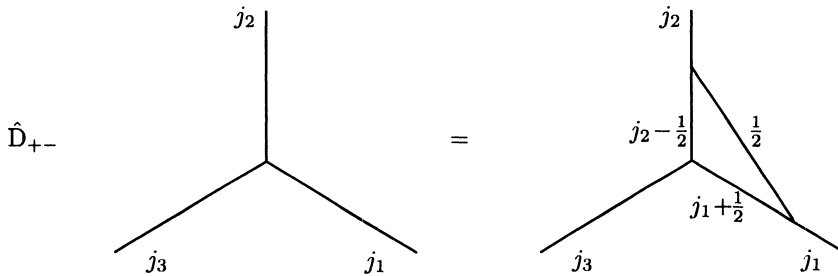
Figure 2: Action of \hat{D}_{i;(IJ)ee'} .
